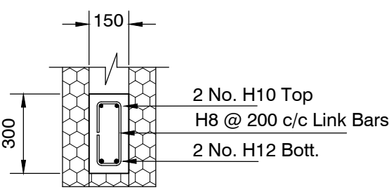
DETAIL RC LINTEL - L1, L8, L11, L14 & L15 Scale 1:20
