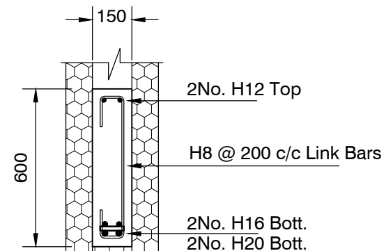
DETAIL RC LINTEL - L7 Scale 1:20
