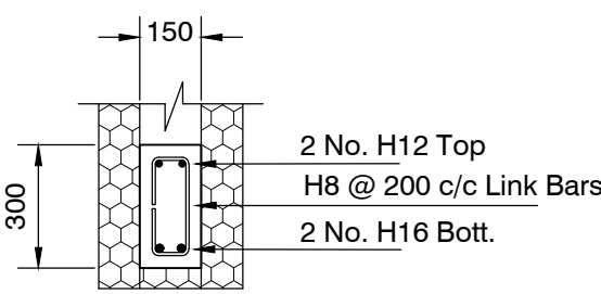
DETAIL RC LINTEL L - 16 Scale 1:20
