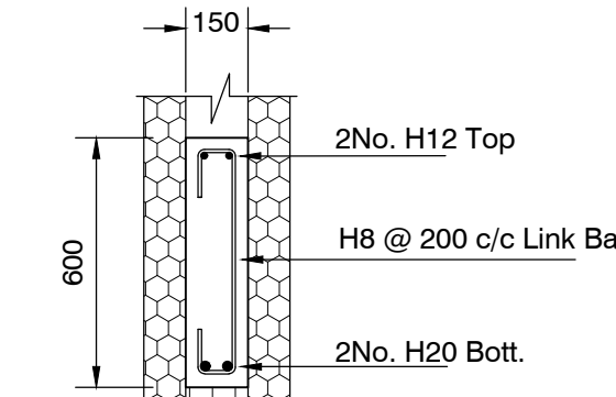
DETAIL RC LINTEL - L13 Scale 1:20
