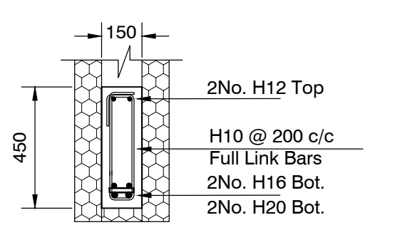
DETAIL RC LINTEL - L6 Scale 1:20
