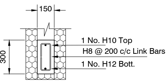
DETAIL RC LINTEL - L2 & L3 Scale 1:20
