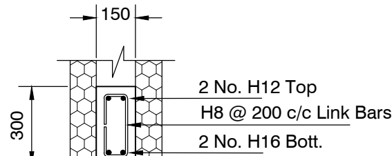
DETAIL RC LINTEL - L9 & L10 Scale 1:20
