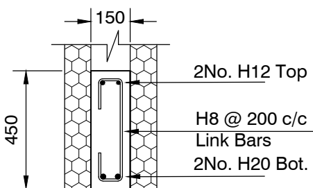
DETAIL RC LINTEL - L4 Scale 1:20
