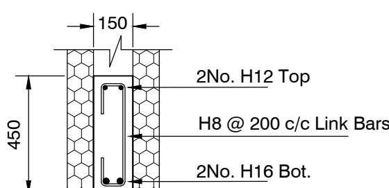
DETAIL RC LINTEL - L5 & L12 Scale 1:20
