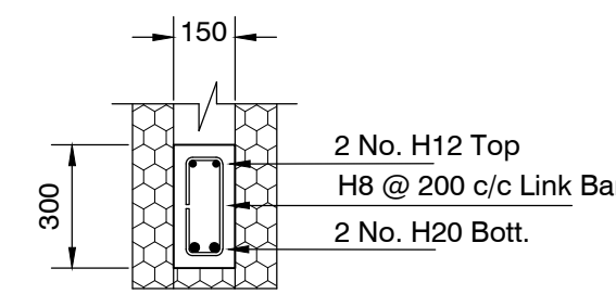
DETAIL RC LINTEL - L17 Scale 1:20
